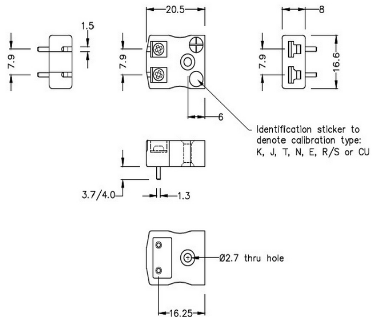
Miniature PCB Socket (dimensions in mm)
