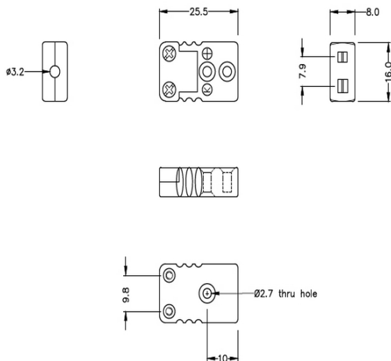
Miniature Hi-Temp Plastic in-line Socket - HTP (dimensions in mm)
